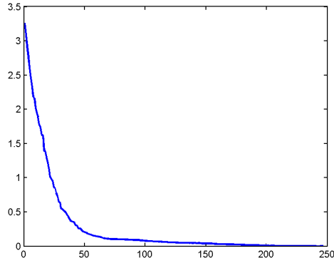
FIG. 4. Plot of \hat{\gamma}(\hat{\lambda}^k) - \gamma_0 as a function of the mixture components k .
