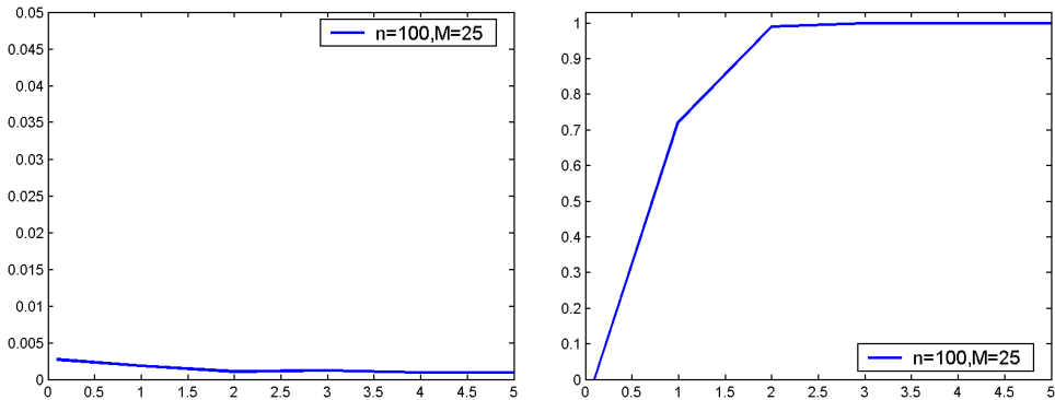
FIG. 3. Dependence on the distance D_{\min} = \min_{k \neq j} |\mu_k - \mu_j| of the L_2 error \|f^* - \hat{f}\|^2 and the percentage of times I^* = \hat{I} . In this example, n = 100 , M = 25 , |I^*| = 2 .
