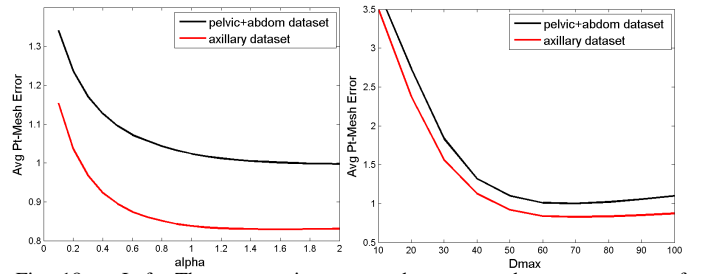
Fig. 18. Left: The symmetric pt-to-mesh error vs the parameter \alpha of the segmentation energy (2). Right: The symmetric pt-to-mesh error vs the parameter D_{max} of (1).
