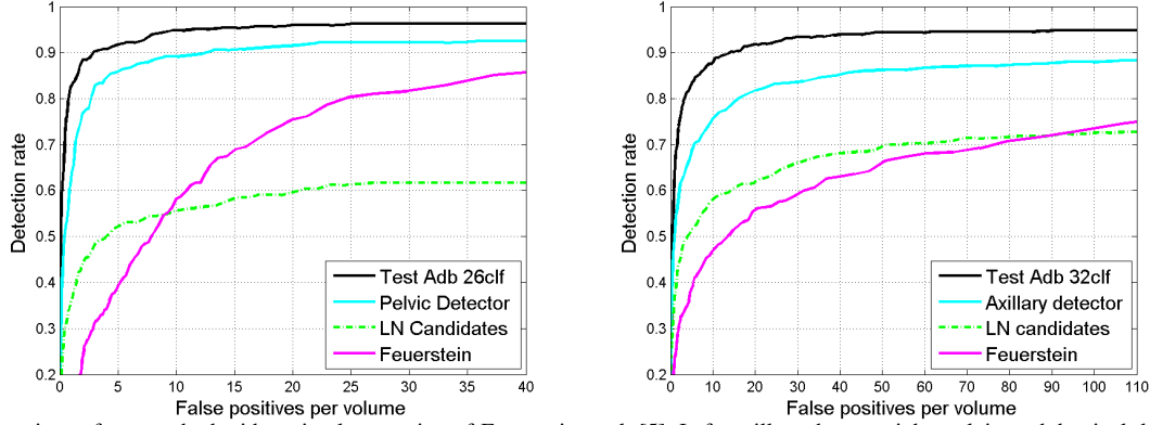
Fig. 17. Comparison of our method with an implementation of Feuerstein et al, [5]. Left: axillary dataset, right: pelvic + abdominal dataset. Also displayed is the performance of the pelvic detector on the axillary dataset (left) and the axillary detector on the pelvic+abdominal dataset (right).
