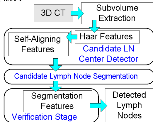
Fig. 1. Diagram of the proposed solid lymph node detection method.
