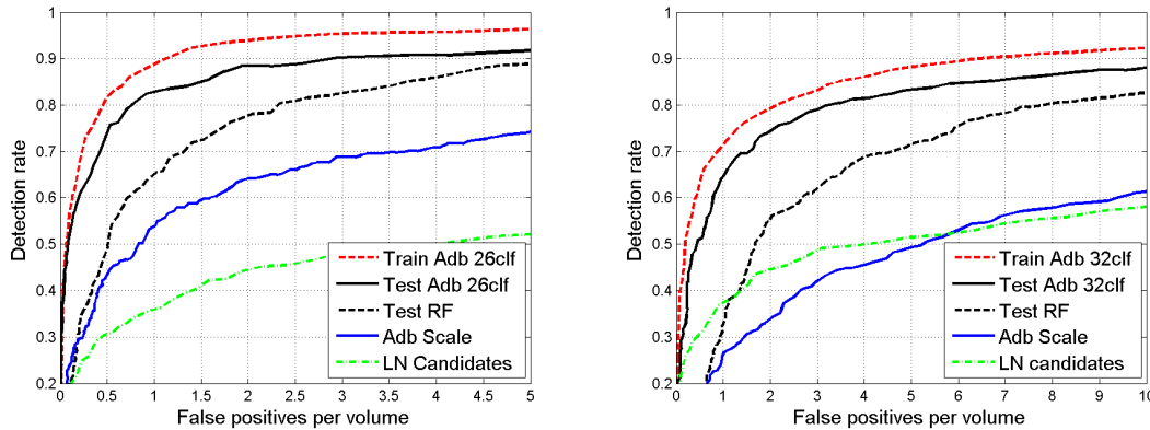
Fig. 16. Lymph node detection results with six-fold cross-validation. Left: Axillary LN evaluation on 131 volumes containing 371 LN. Right: Pelvic and abdominal LN evaluation on 54 volumes containing 569 LN.
