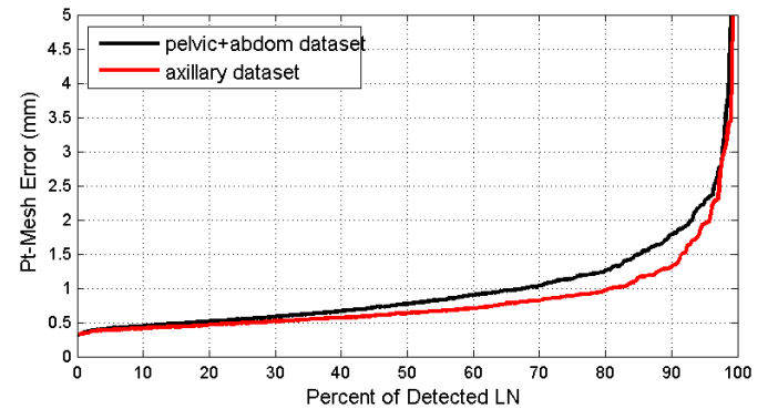
Fig. 19. The sorted point-to-mesh errors for the two datasets being evaluated.
