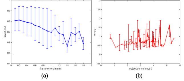
Figure 7. Statistics of errors (mm) on the evaluation set for the ARO method: (a) The likelihood (Eq.(5)) versus frame errors and each bar shows max/min likelihood values; (b) Sequence errors (mean and error bar) versus log(sequence length).
