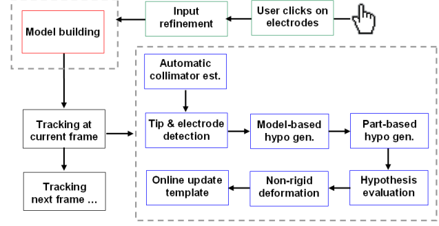
Figure 2. A block diagram of our proposed approach.
