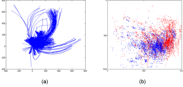
Figure 6. Illustration of our CS catheter dataset: (a) Catheter shapes after aligning to PCS; (b) Distribution of tips (red) and PCS (blue).
